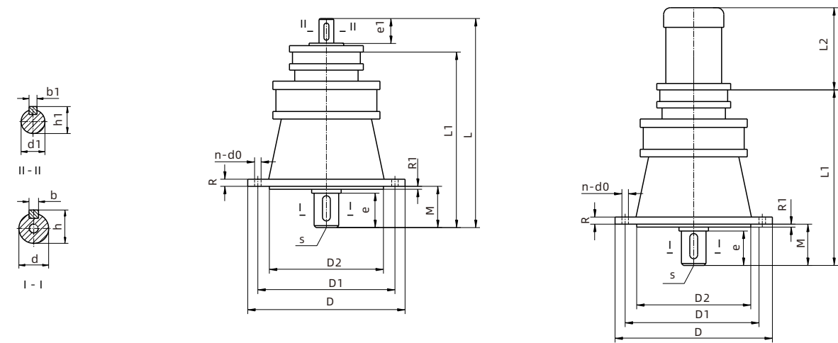
6、WBLE(WBLED)型立式双级摆线减速机外型及安装尺寸 WBLE(WBLED)type vertical double-stage cycloidal speed reducer appearance and installation dimension
