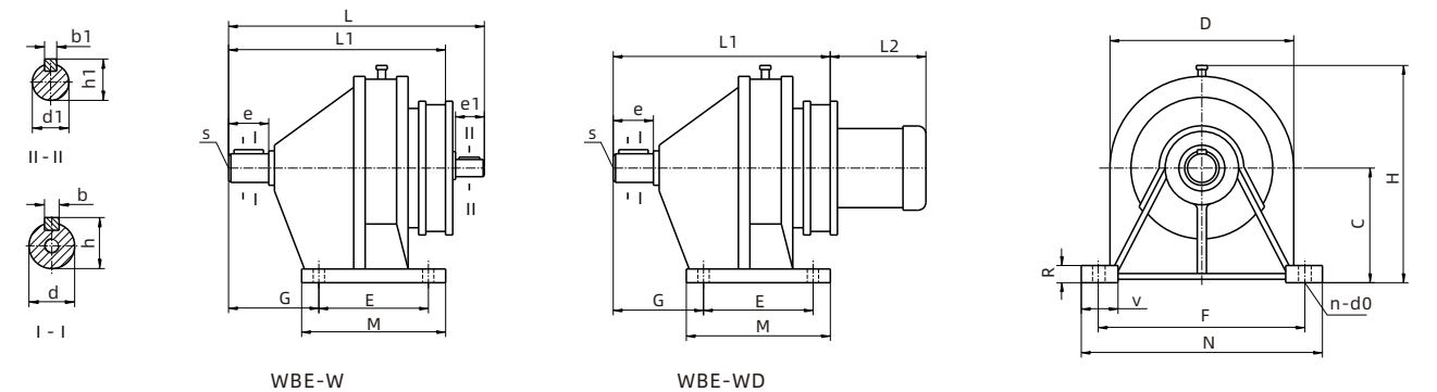
5、WBE(WBED)型卧式双级摆线减速机外型及安装尺寸 WBE(WBED)type horizontal double cycloidal speed reducer appearance installation dimension
