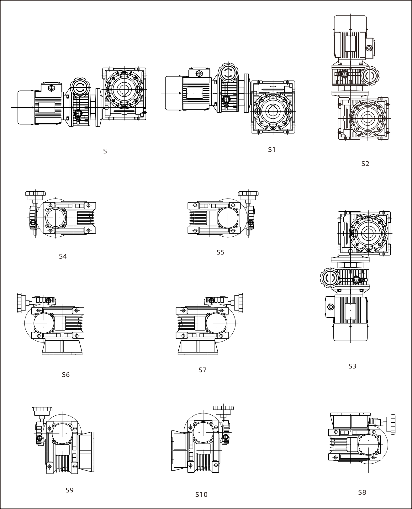
The unit of variator plus worm microreducer structure and mounting position code
