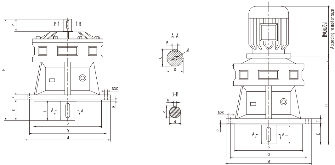
九.BL、BLD、XL、XLD型(单级)外形及安装尺寸 Model BL、BLD、XL、XLD (single reduction) contour and installation dimension
