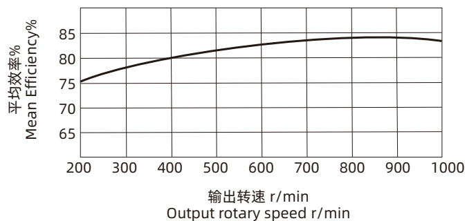
标准型平均效率与输出转速的关系 Relation between the standard-type's mean efficiency and the output rotary speed
