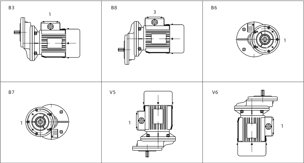
PC系列减速机安装方式 Mounting Position of PC Series Gear Reducer
