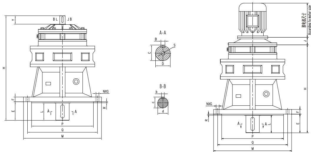
十一.BLE、BLED、XLE、XLED型(双级)外形及安装尺寸 Model BLE、BLED、XLE、XLED (double reduction) contour and installation dimension
