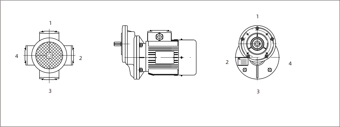
电机接线盒方向 Location of terminal box
